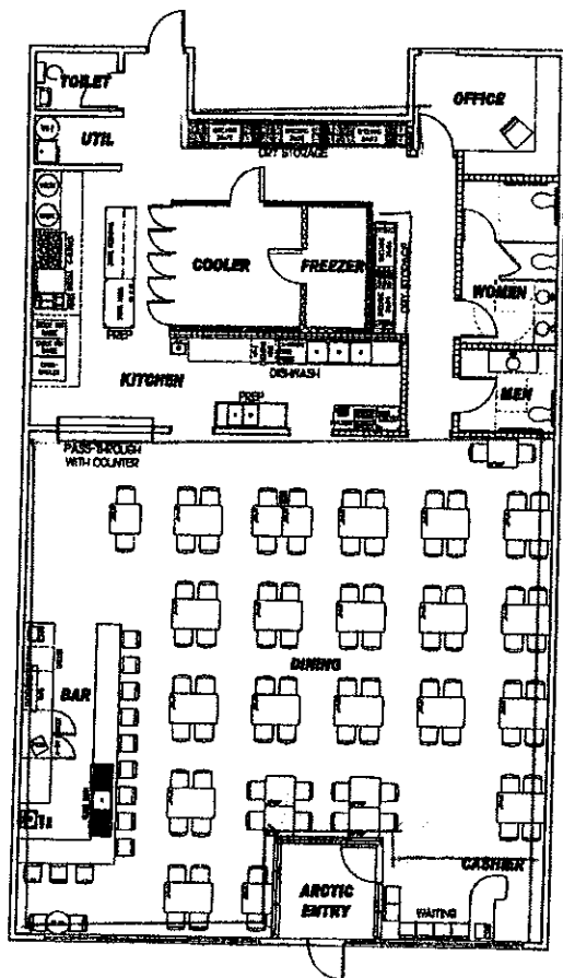
2 FLOOR PLAN - NEW SHP-1-C
